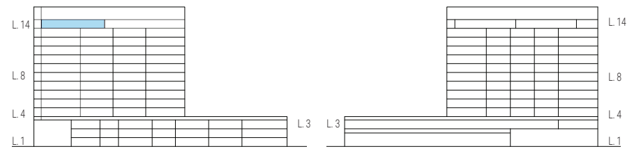
SOUTH ELEVATION
